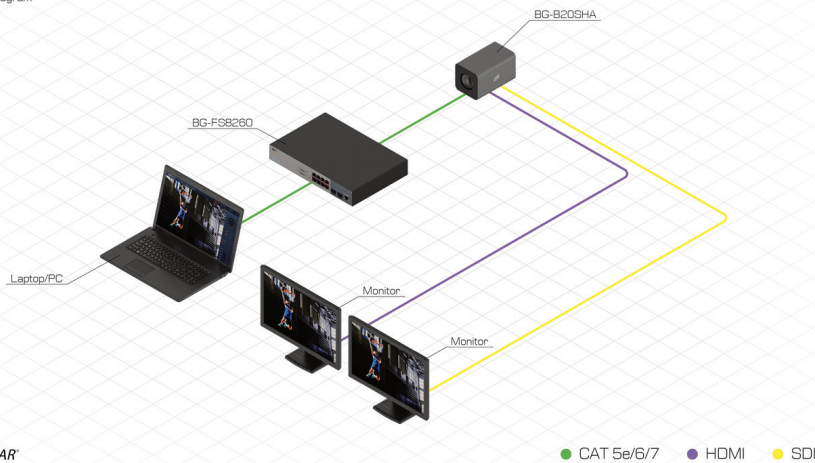
BG-B20SHA Connection Diagram
