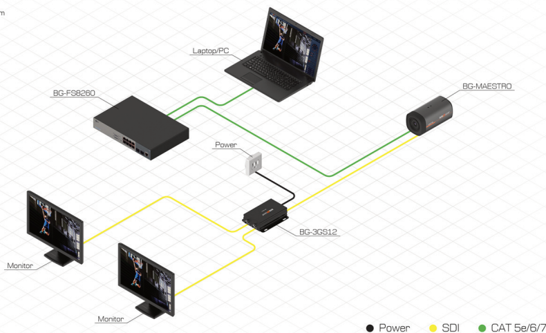
BG-Maestro Connection Diagram
