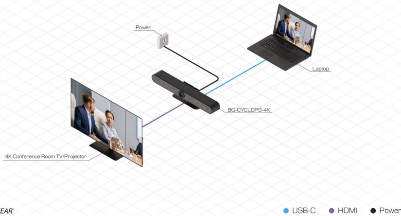
BG-CYCLOPS-4K Connection Diagram
