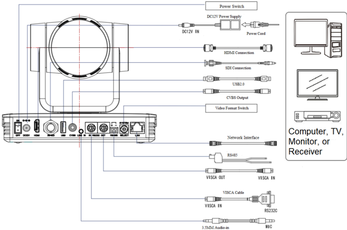
Wiring Diagram
