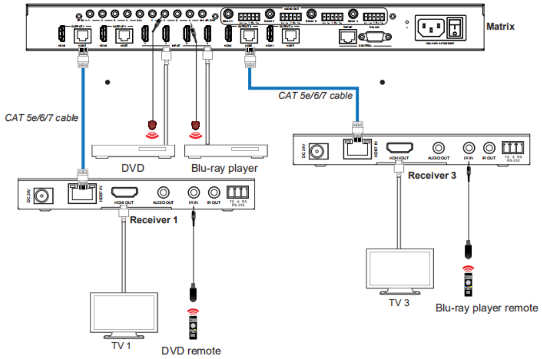
Figure 2: IR connection diagram (HDBaseT Receiver end)
