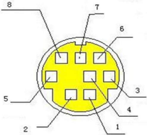
RS-232 Mini-DIN 8-pin Port Definition
