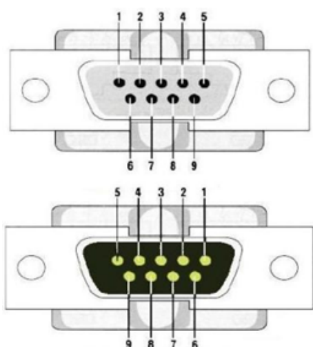
RS-232 (BD9) Port Connections
