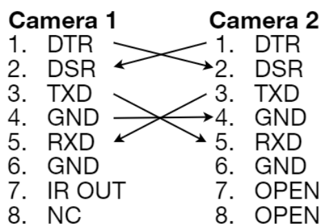
Camera cascade connection
