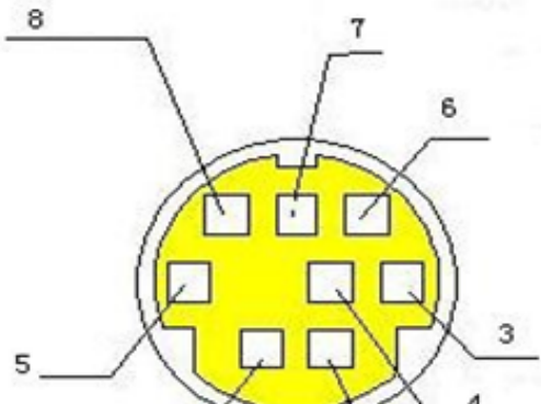
RS-232 Mini-DIN 8-pin Port Definition
